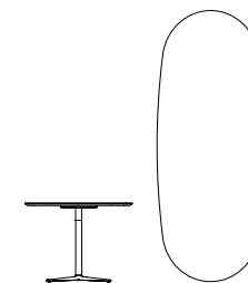
PARTNERSHIP conference table 2300 × 1000 × 740 mm (L × W × H)
