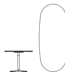
PARTNERSHIP conference table 2100 × 1000 × 740 mm (L × W × H)
