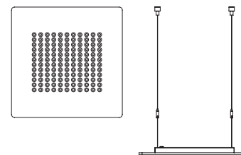
Silurus-Ply lamp 400 x 400 x max. 900 mm (LxWxH)
