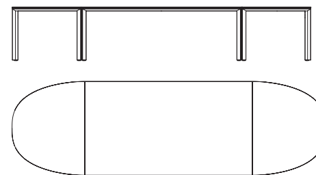
Admiral bespoke modular boardroom table 4300 × 1290 × 745 mm (L × W × H)
