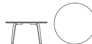
SUBMARINE large round coffee table Ø800 × 430 mm (D×H)
