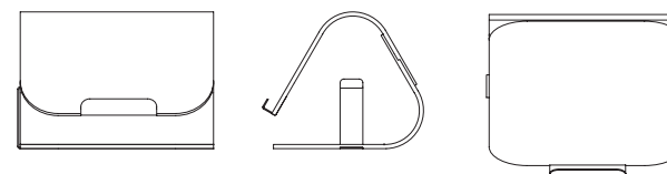
PILOT kitchen roll holder and tablet stand 260 × 213 × 182 mm (L×W×H)
