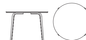
MOTHERSHIP large round tea table Ø1200 × 750 mm (D × H)
